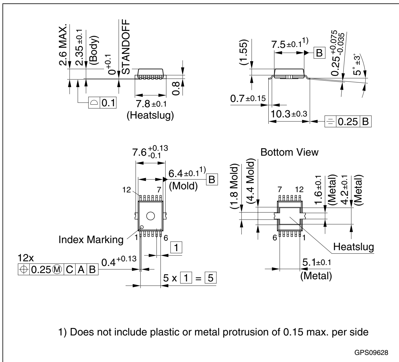
Figure 9 PG-DSO-12 (Plastic Green Dual Small Outline)
